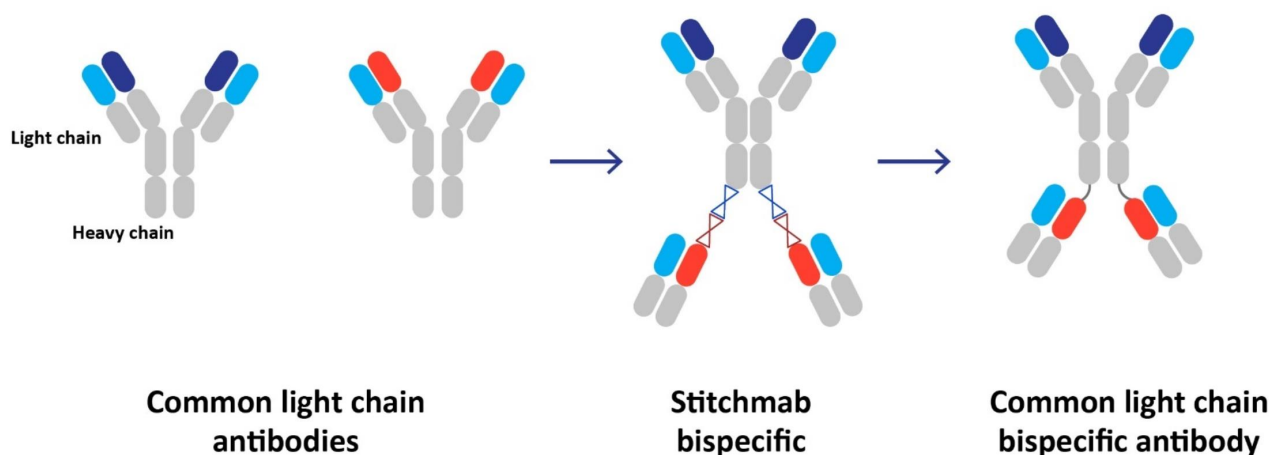
Figure 2. A common light chain simplifies the production of bispecific antibodies
